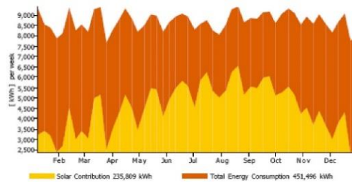
Fig 10. (a) Solar energy analysis draft/ Source: Author (from KRGIT)
