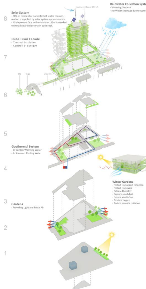
Fig 11. (a) Application of renewal energies in a green high rise building/ Source: Author (from KRGIT)
