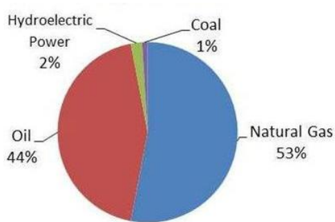
Fig 5. Energy mix in Iran, Source: www.citic.ir
